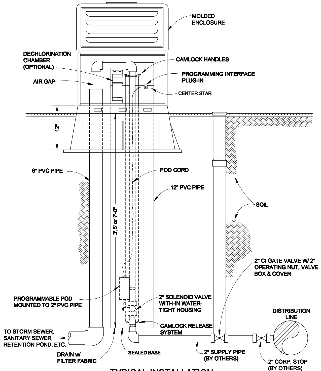
TYPICAL INSTALLATION HYDRO-GUARD HG-4
